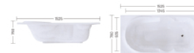
WBT-005 Length 1525mm Breadth 760mm Depth 405mm Waste Hole Distance from wall 350mm
